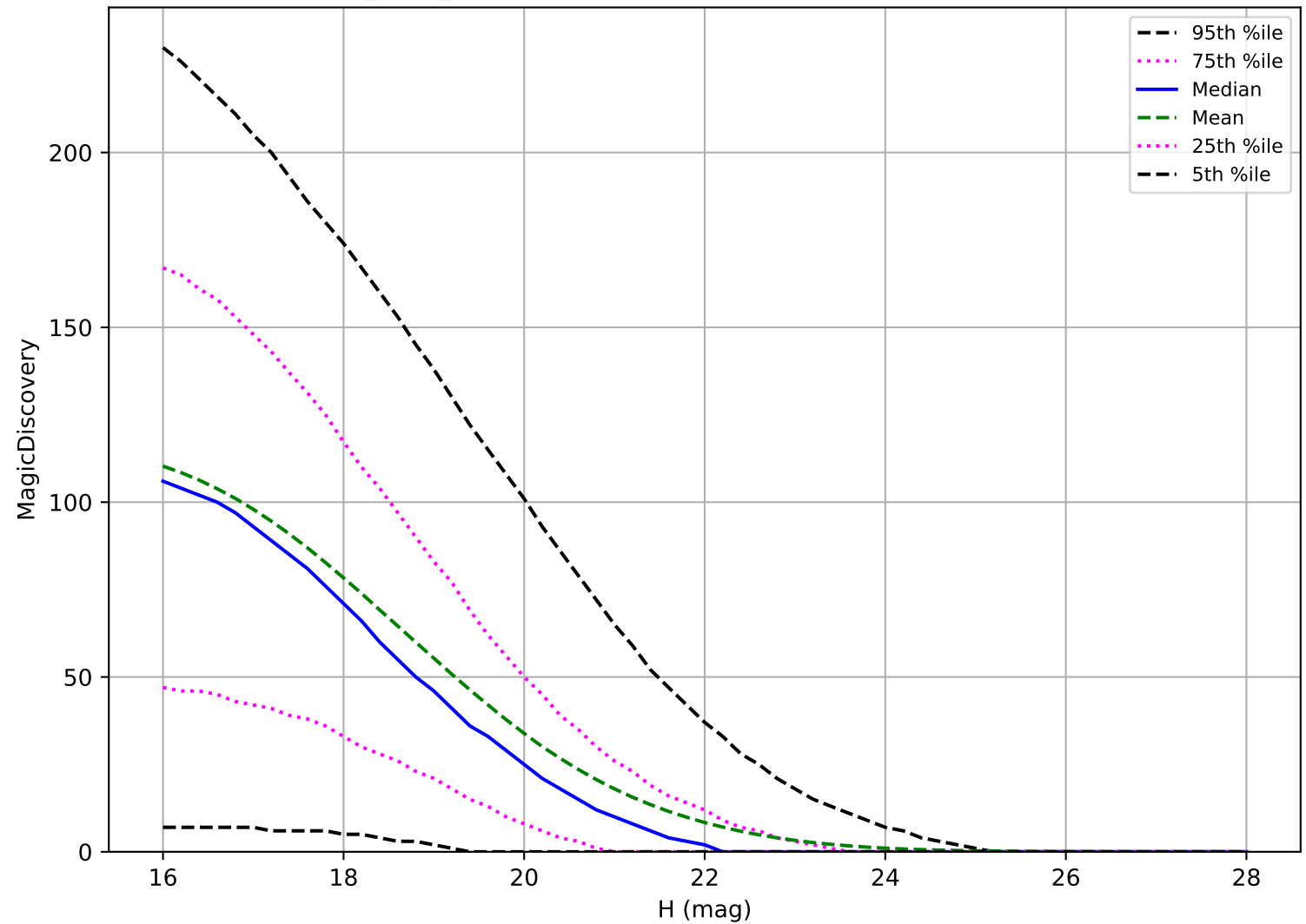
baseline_v3.2_10yrs: PHA 6 detections in 60 nights detection loss
