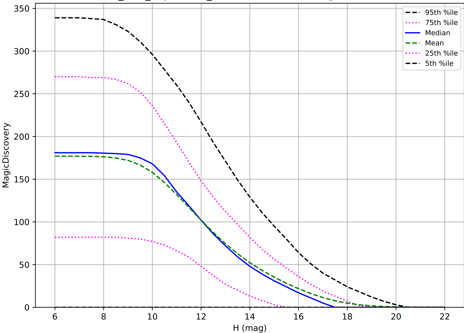
baseline_v3.2_10yrs: OCC_r5 6 detections in 60 nights detection loss
