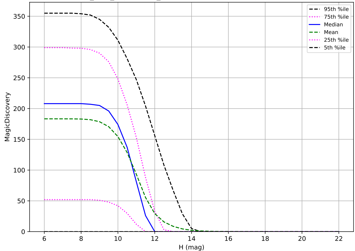
baseline_v3.2_10yrs: OCC_r20 6 detections in 60 nights detection loss
