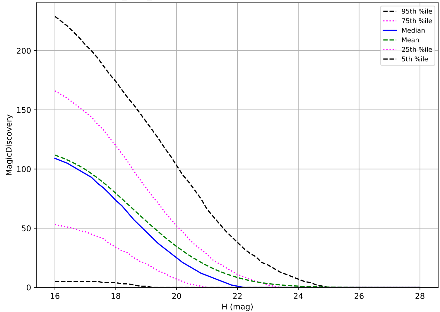
baseline_v3.2_10yrs: NEO 6 detections in 60 nights detection loss
