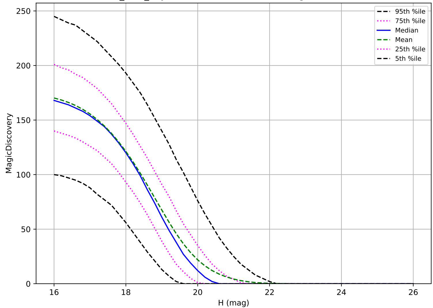
baseline_v3.2_10yrs: MBA 6 detections in 60 nights detection loss
