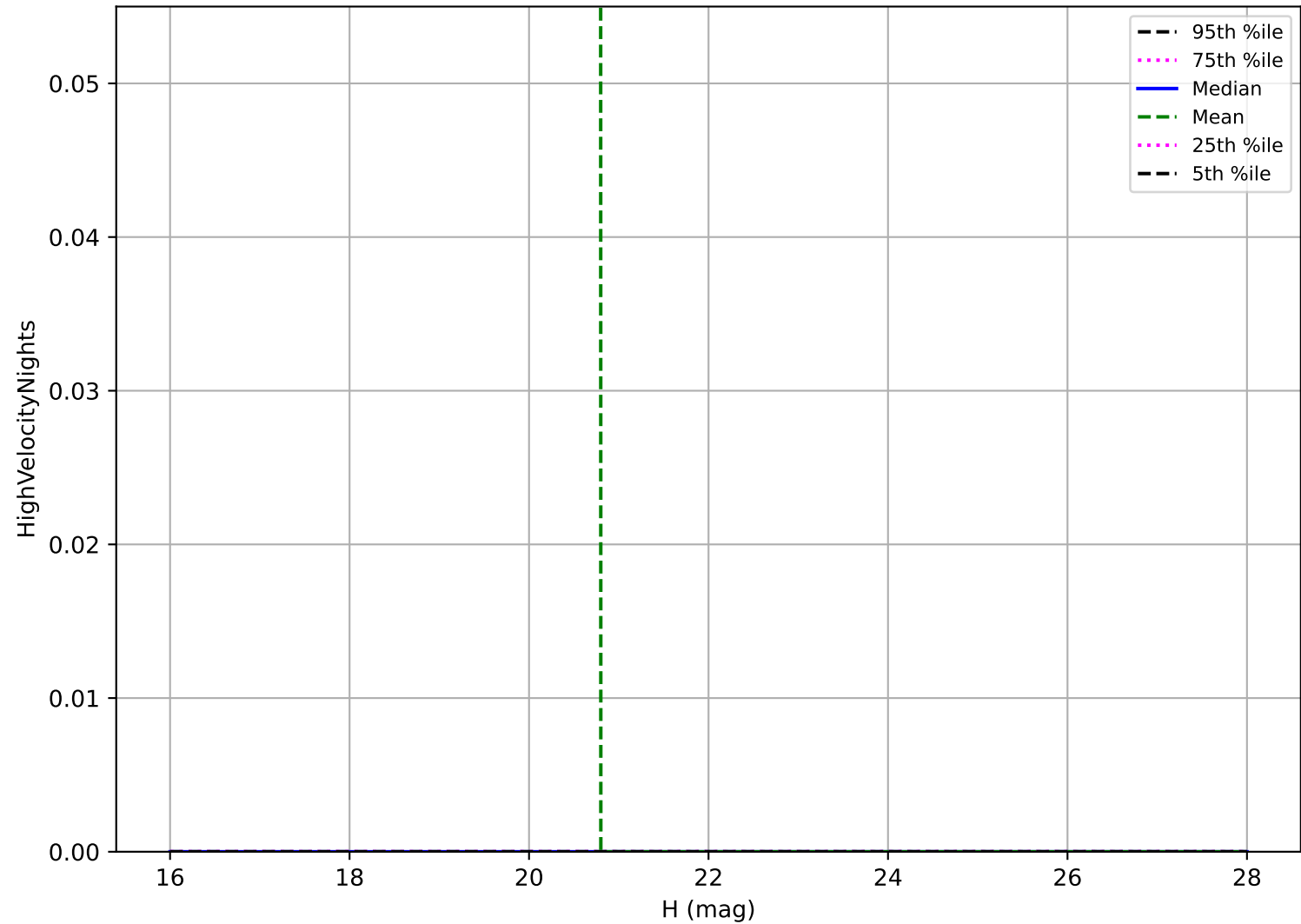
baseline_v3.2_10yrs: Vatira High velocity pair detection loss
