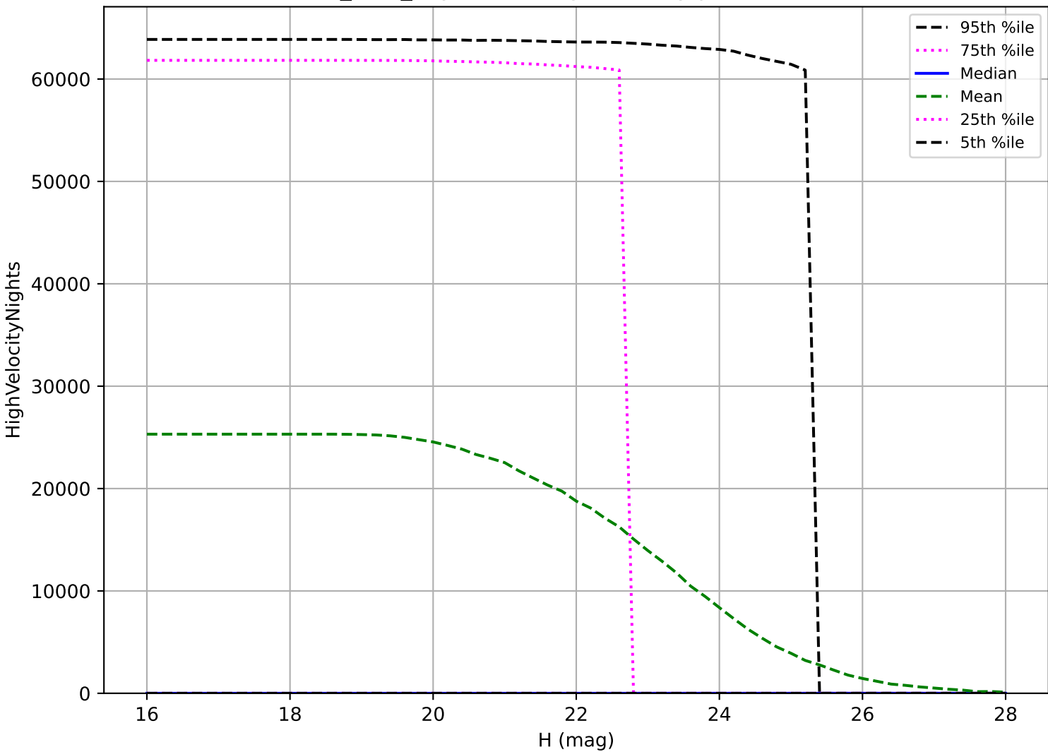
baseline_v3.2_10yrs: PHA High velocity pair detection loss
