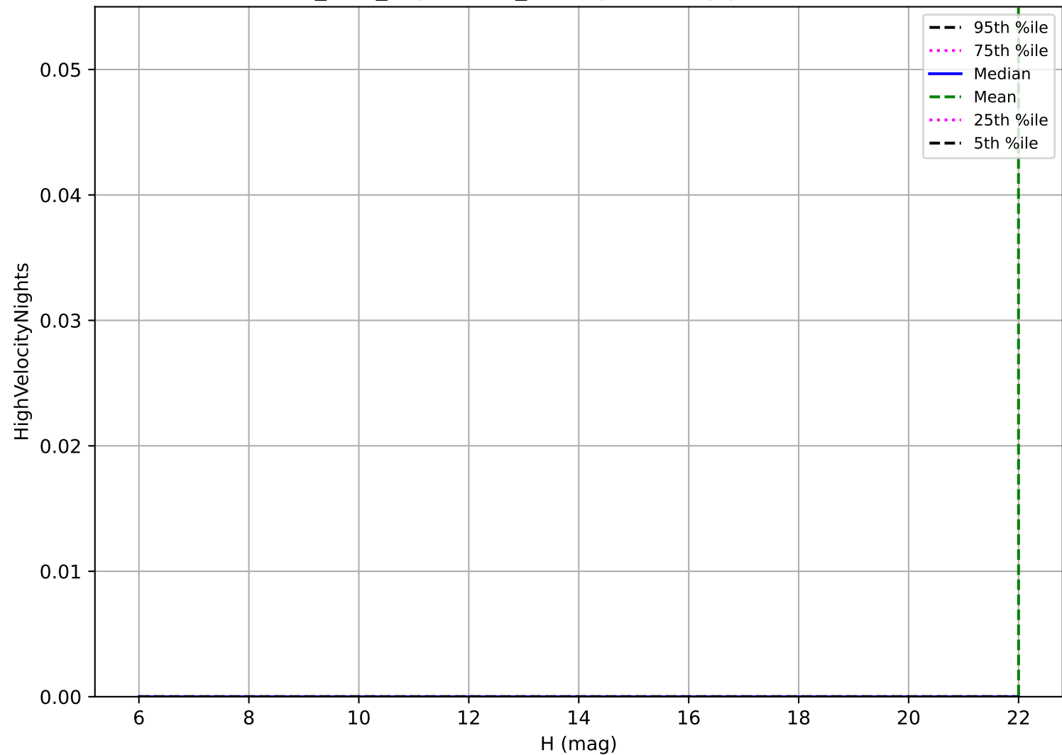
baseline_v3.2_10yrs: OCC_r20 High velocity pair detection loss
