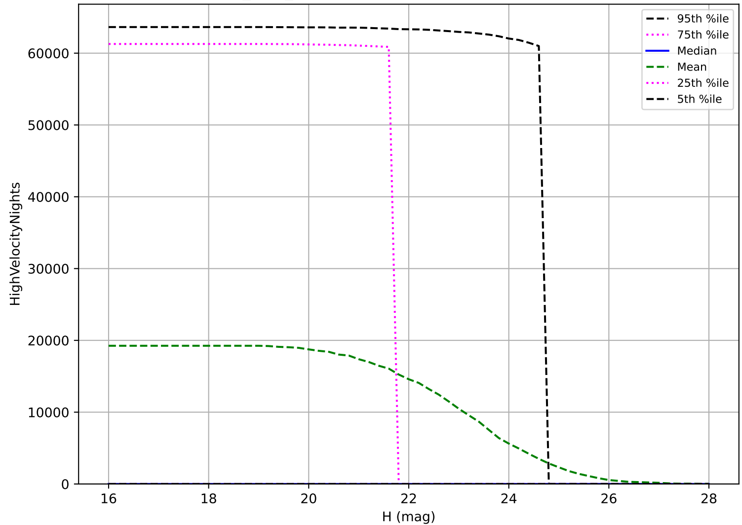
baseline_v3.2_10yrs: NEO High velocity pair detection loss
