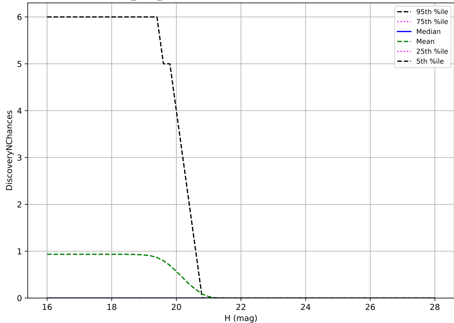
baseline_v3.2_10yrs: Vatira 3 pairs in 15 nights detection loss
