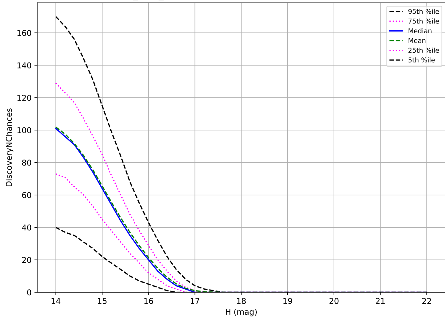
baseline_v3.2_10yrs: Trojan 3 pairs in 15 nights detection loss
