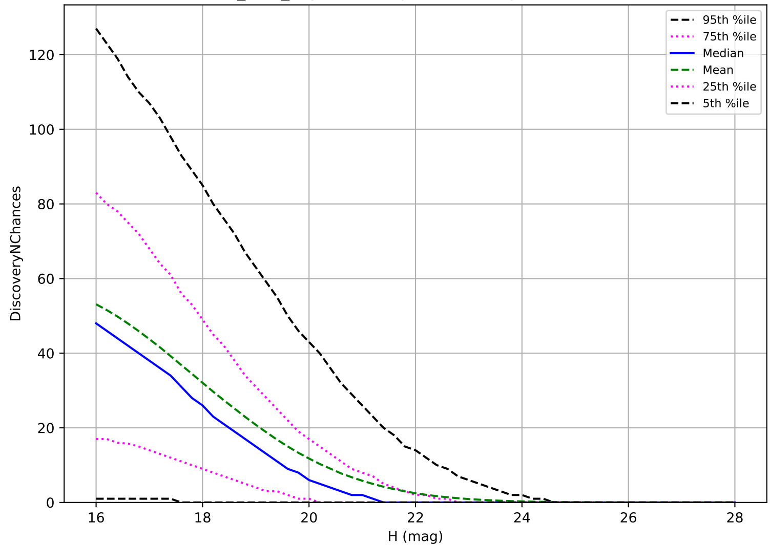
baseline_v3.2_10yrs: PHA 3 pairs in 15 nights detection loss
