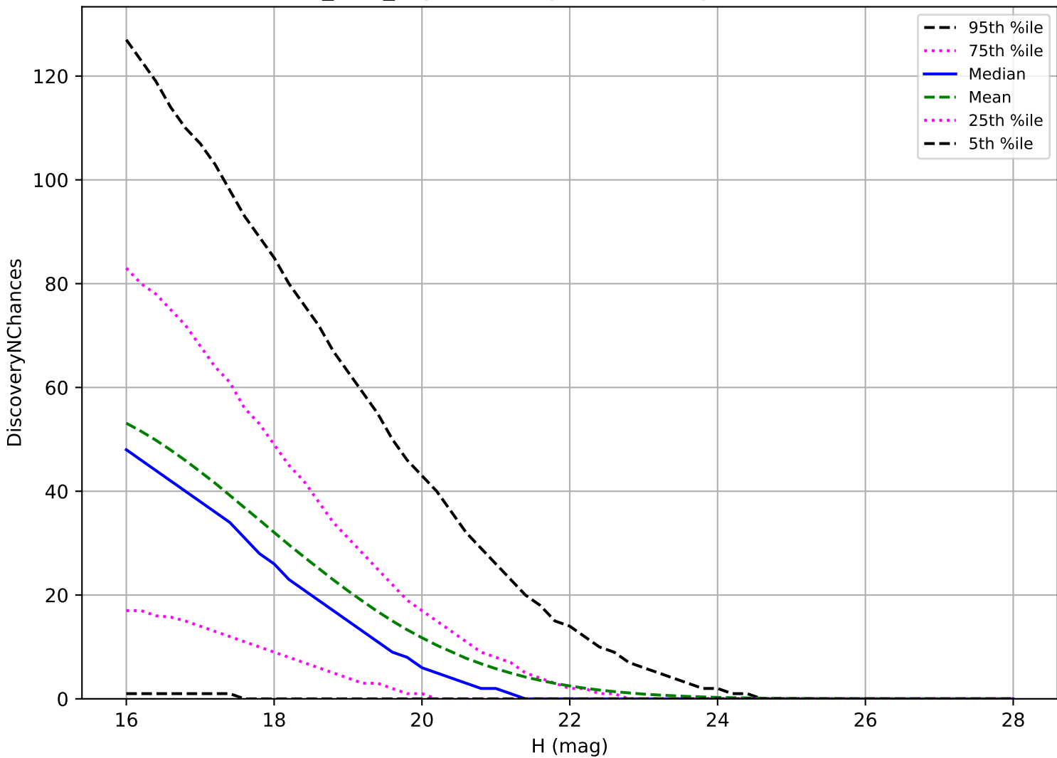
baseline_v3.2_10yrs: PHA 3 pairs in 15 nights detection loss
