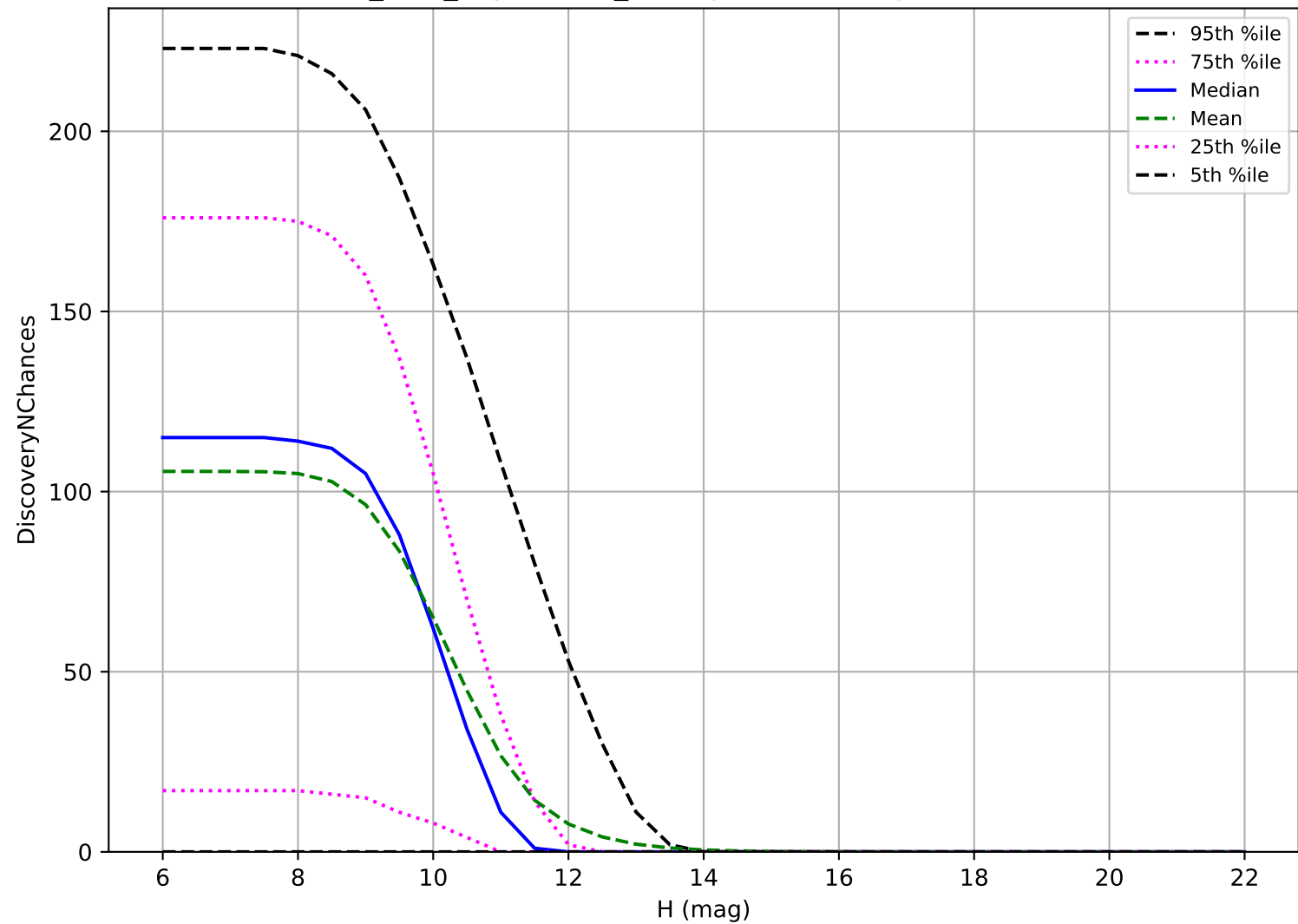
baseline_v3.2_10yrs: OCC_r20 3 pairs in 15 nights detection loss
