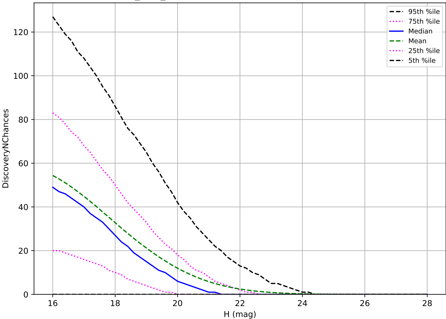
baseline_v3.2_10yrs: NEO 3 pairs in 15 nights detection loss
