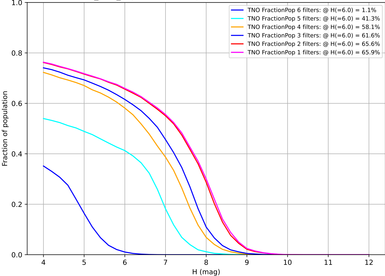
baseline_v3.2_10yrs: Fraction of population with colors in X filters TNO
