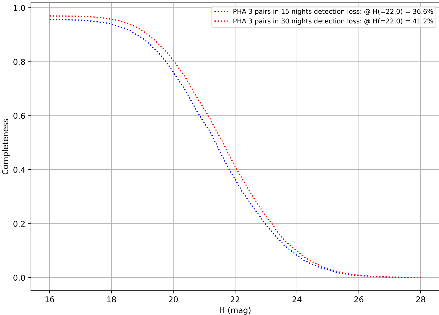
baseline_v3.2_10yrs: DifferentialCompleteness
