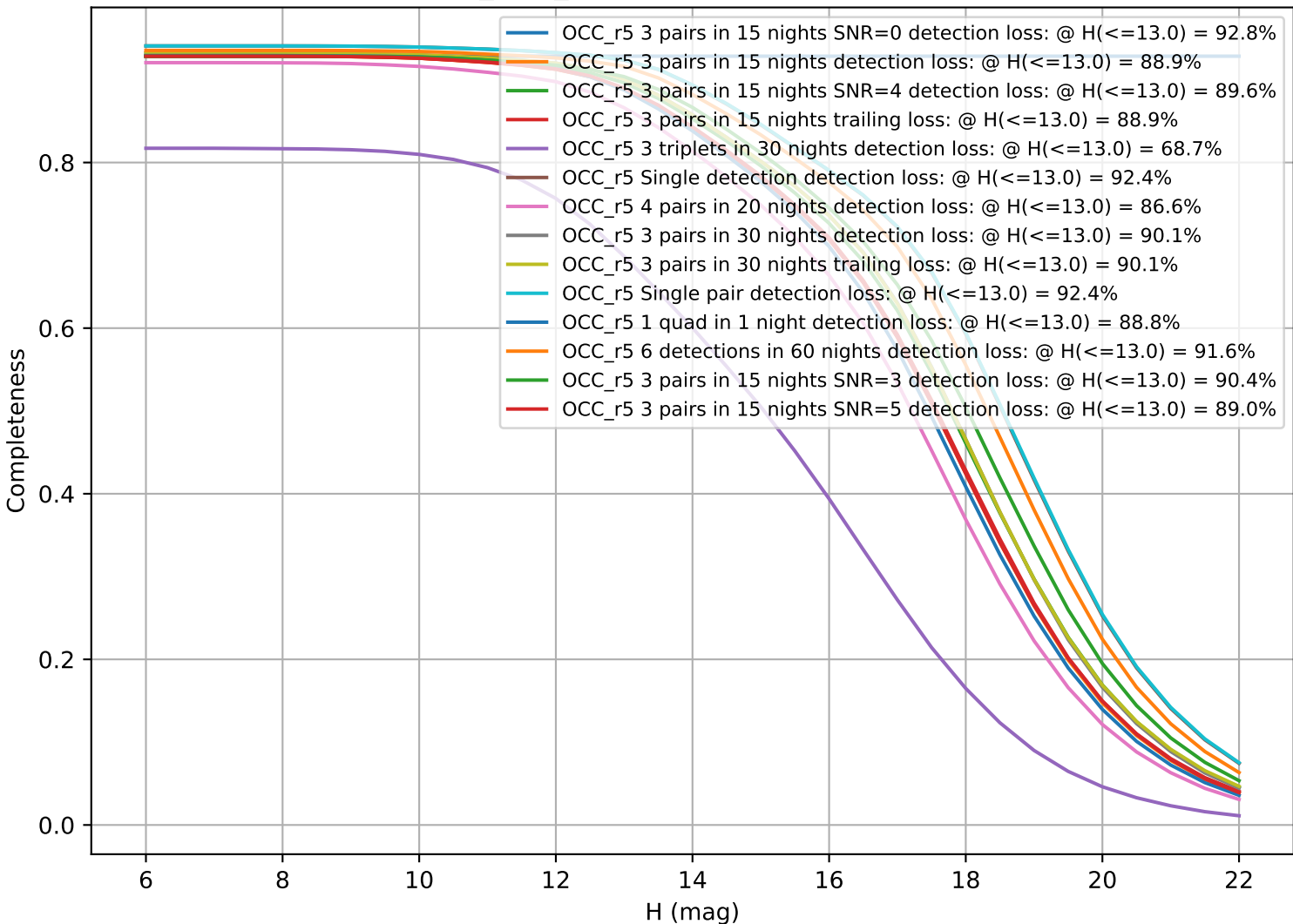
baseline_v3.2_10yrs: CumulativeCompleteness
