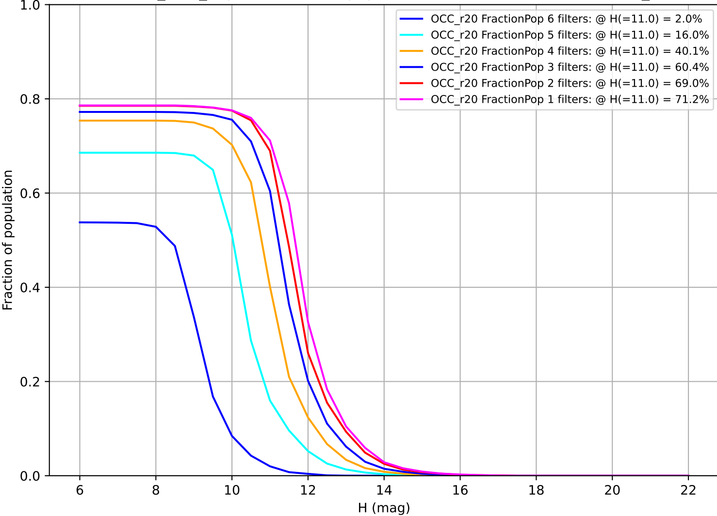
baseline_v3.2_10yrs: Fraction of population with colors in X filters OCC_r20
