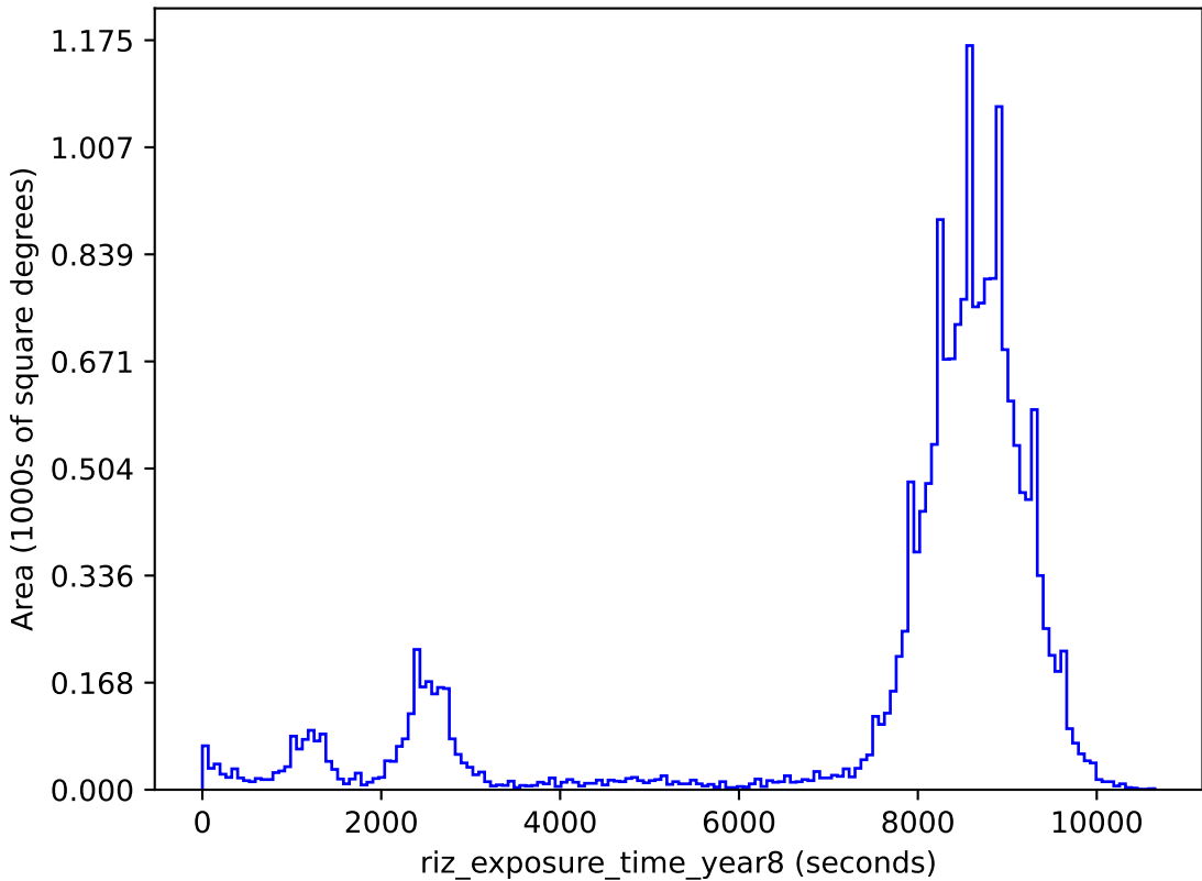
baseline_v3.2_10yrs gri band non-DD: riz_exposure_time_year8
