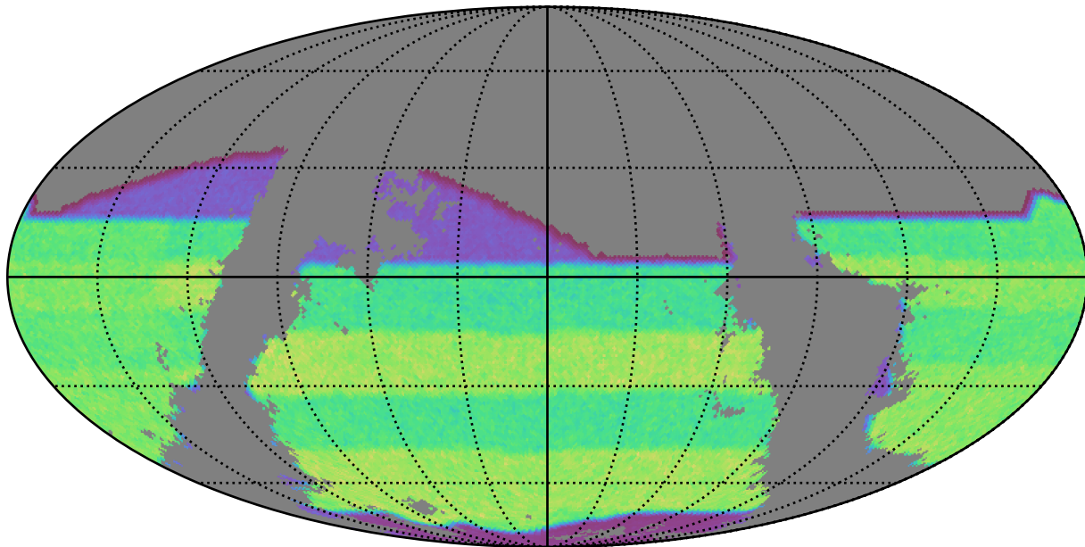
baseline_v3.2_10yrs gri band non-DD: riz_exposure_time_year7
