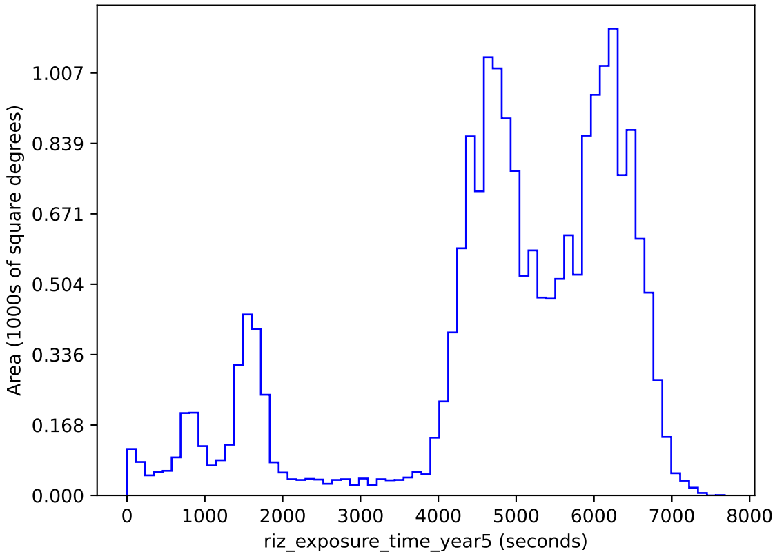
baseline_v3.2_10yrs gri band non-DD: riz_exposure_time_year5
