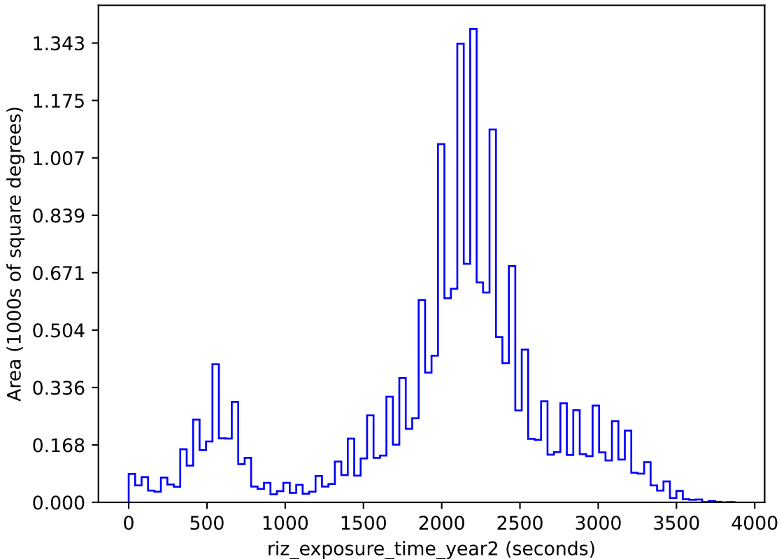
baseline_v3.2_10yrs gri band non-DD: riz_exposure_time_year2
