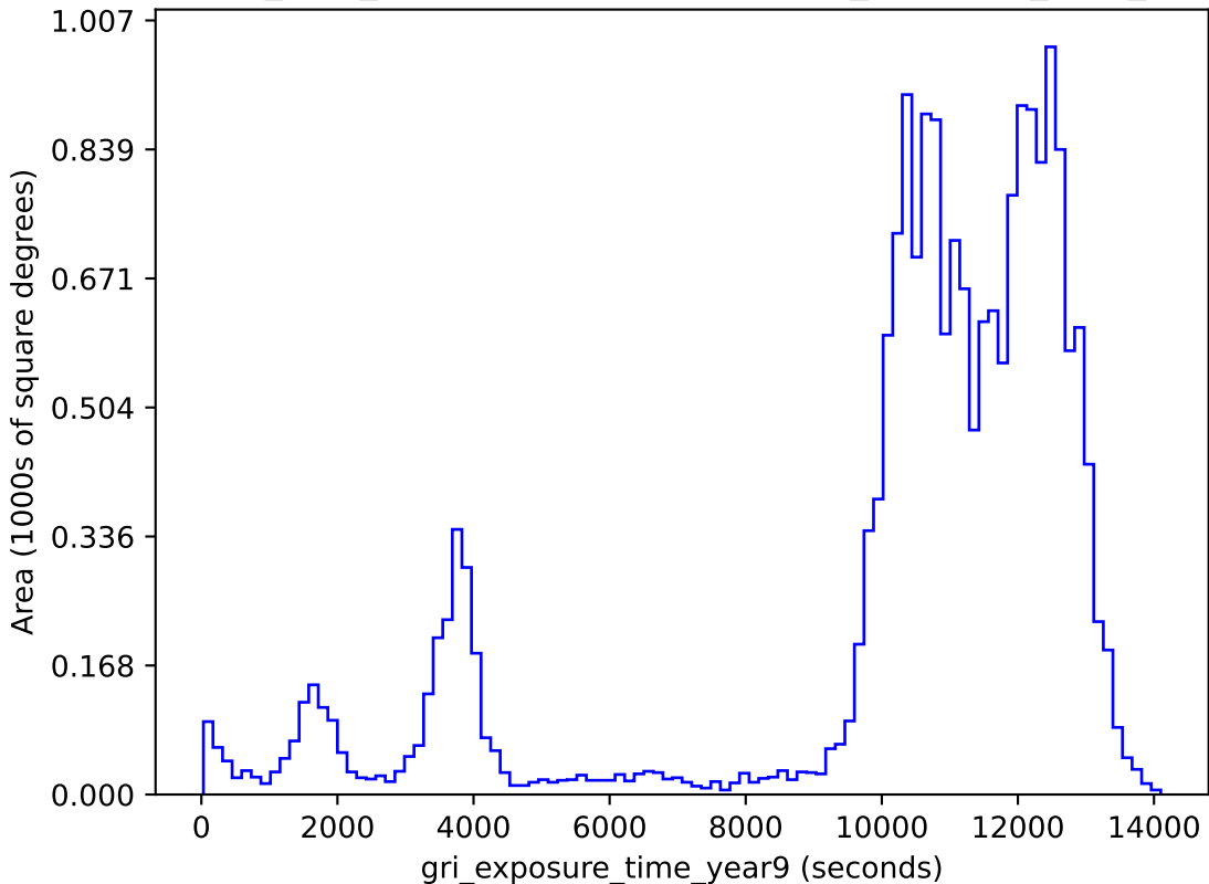
baseline_v3.2_10yrs gri band non-DD: gri_exposure_time_year9
