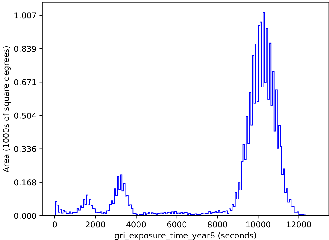
baseline_v3.2_10yrs gri band non-DD: gri_exposure_time_year8
