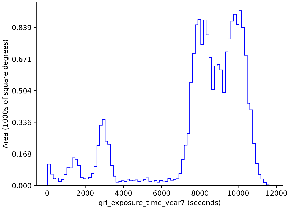
baseline_v3.2_10yrs gri band non-DD: gri_exposure_time_year7
