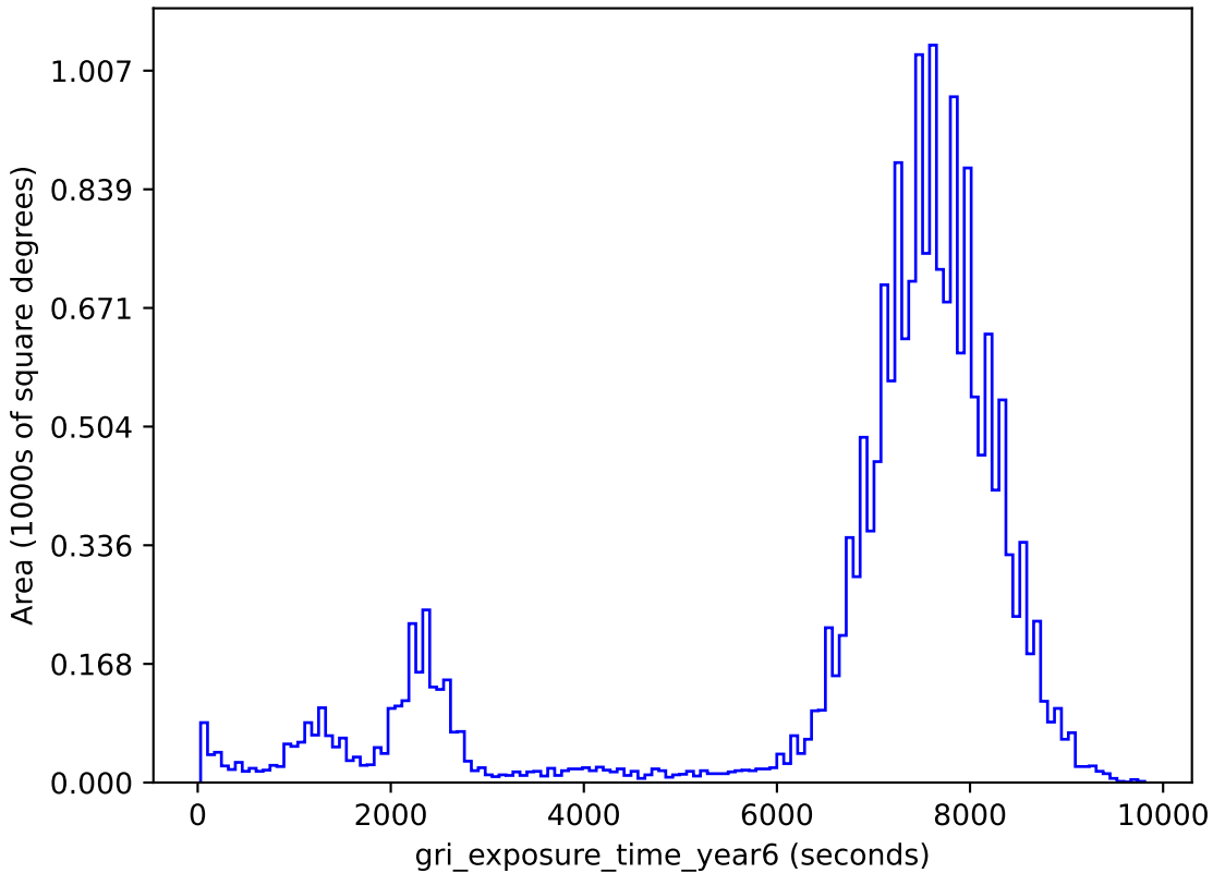
baseline_v3.2_10yrs gri band non-DD: gri_exposure_time_year6
