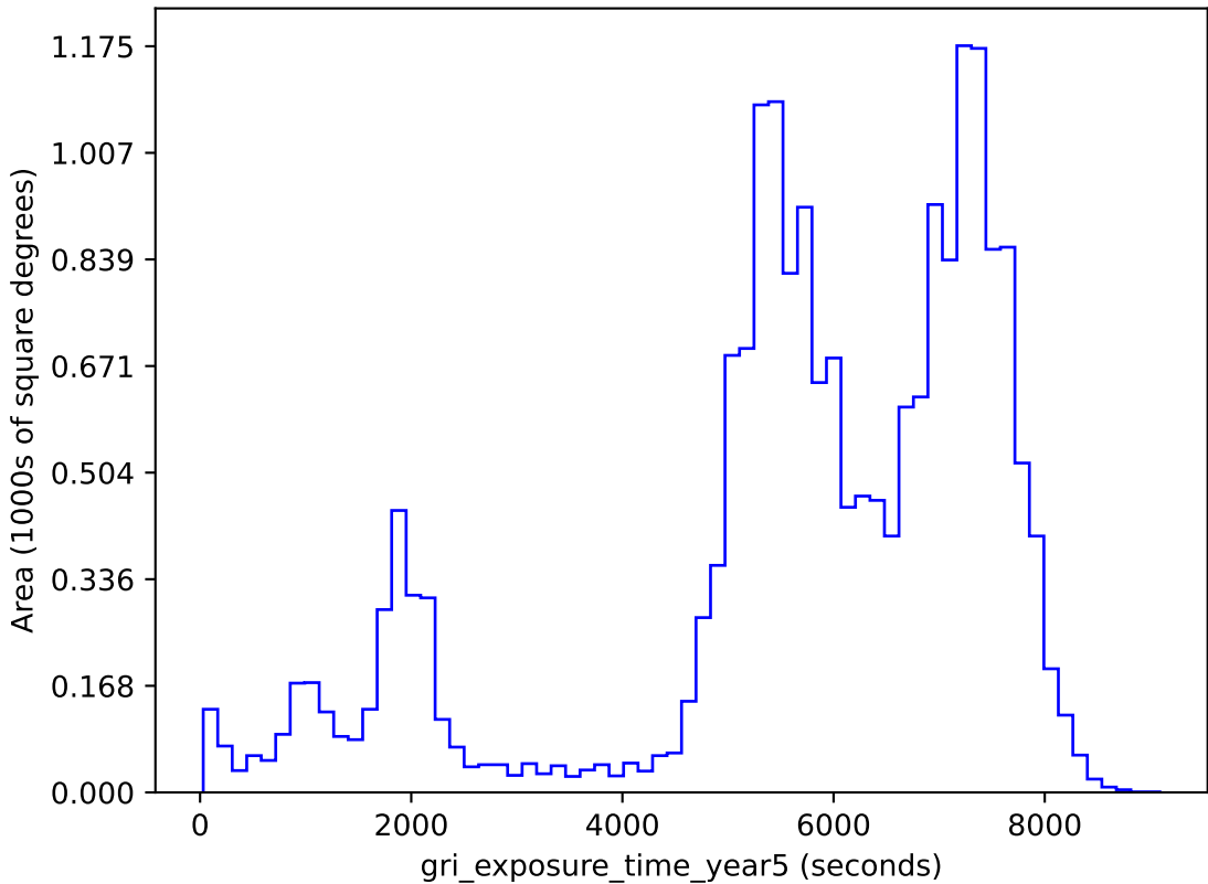
baseline_v3.2_10yrs gri band non-DD: gri_exposure_time_year5
