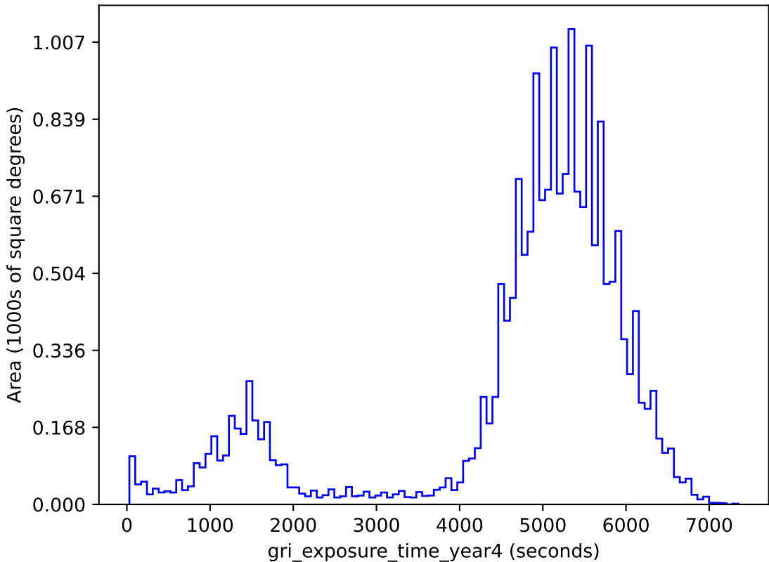
baseline_v3.2_10yrs gri band non-DD: gri_exposure_time_year4
