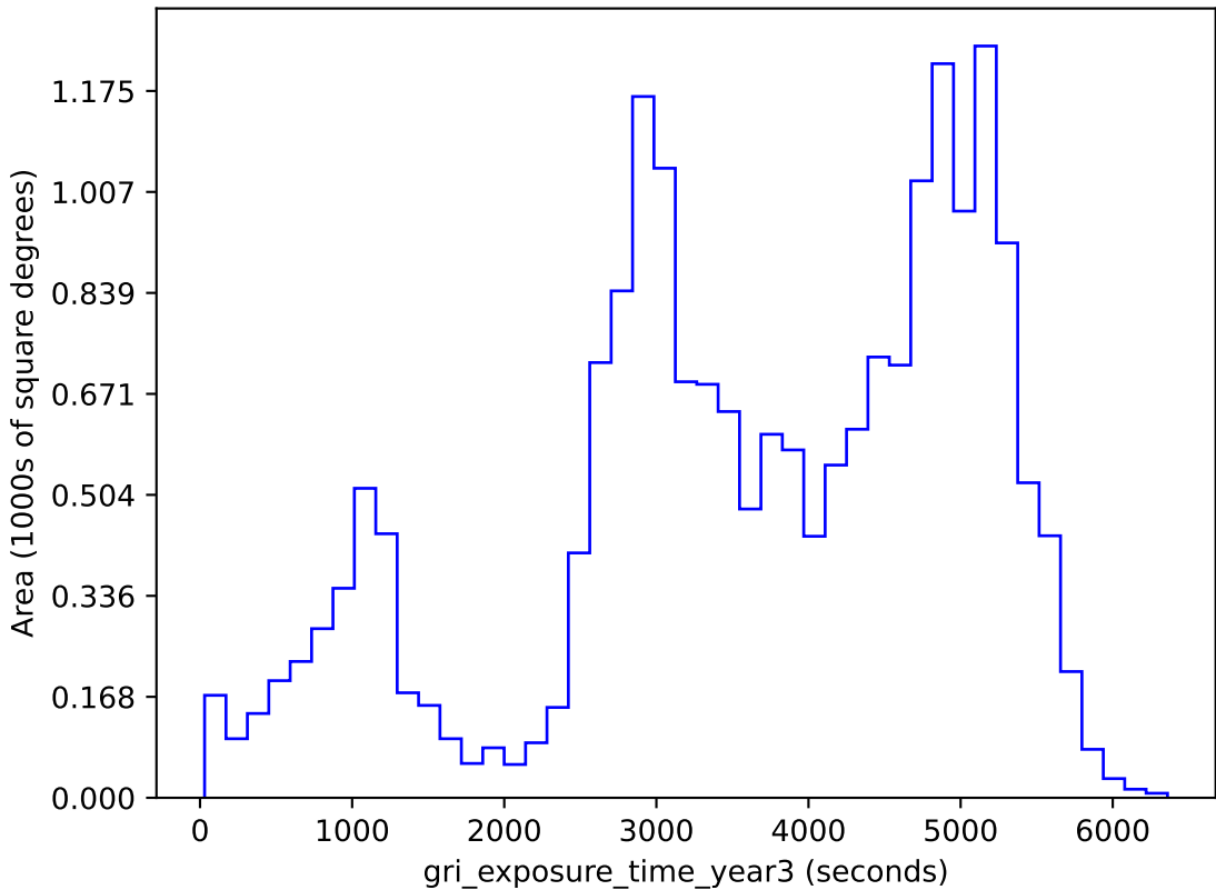
baseline_v3.2_10yrs gri band non-DD: gri_exposure_time_year3
