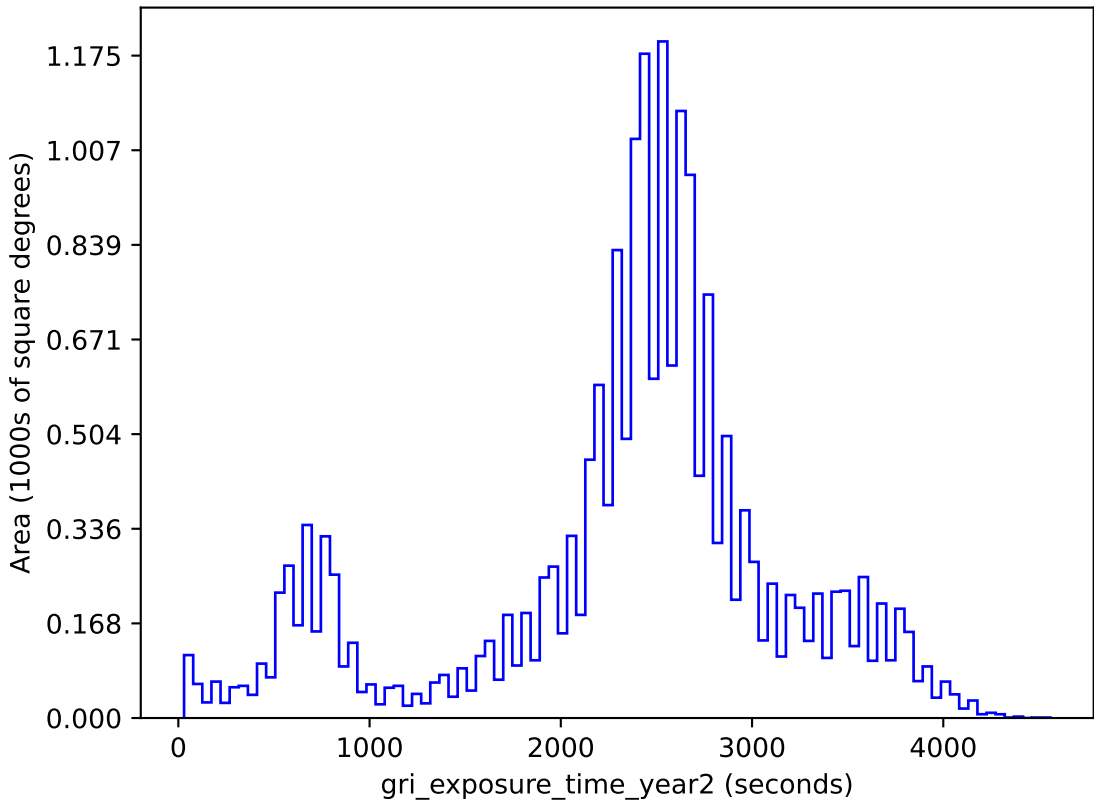
baseline_v3.2_10yrs gri band non-DD: gri_exposure_time_year2
