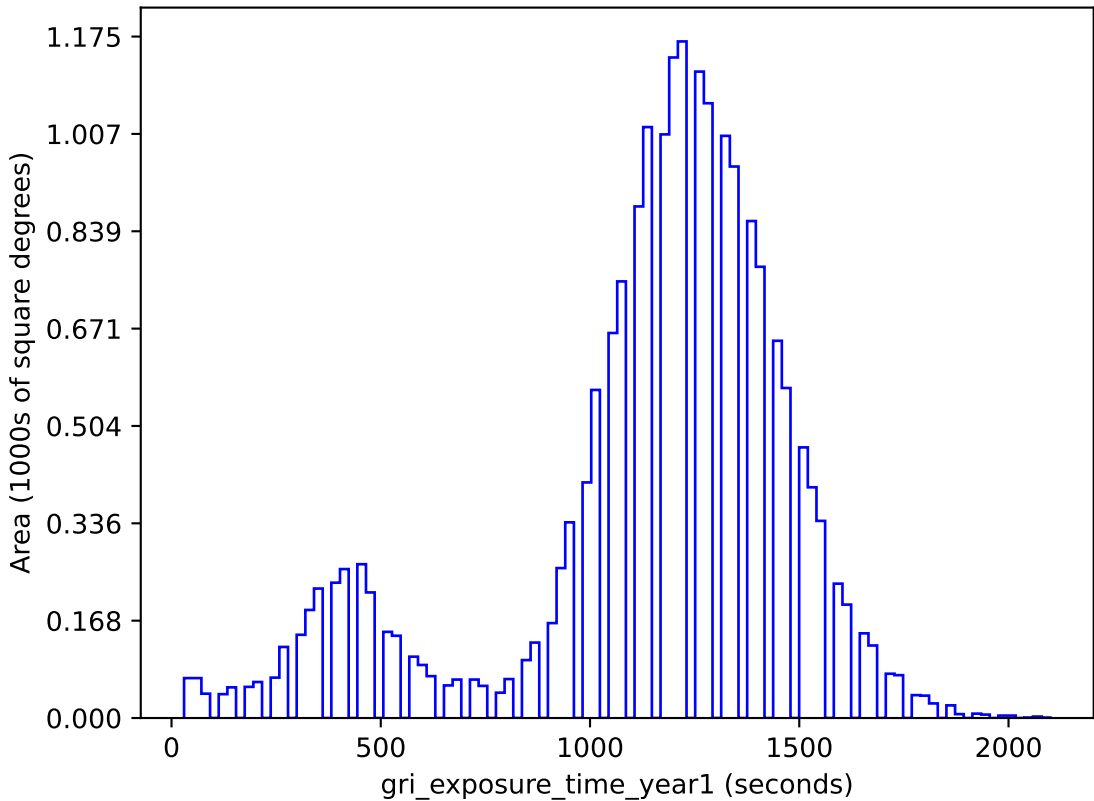
baseline_v3.2_10yrs gri band non-DD: gri_exposure_time_year1
