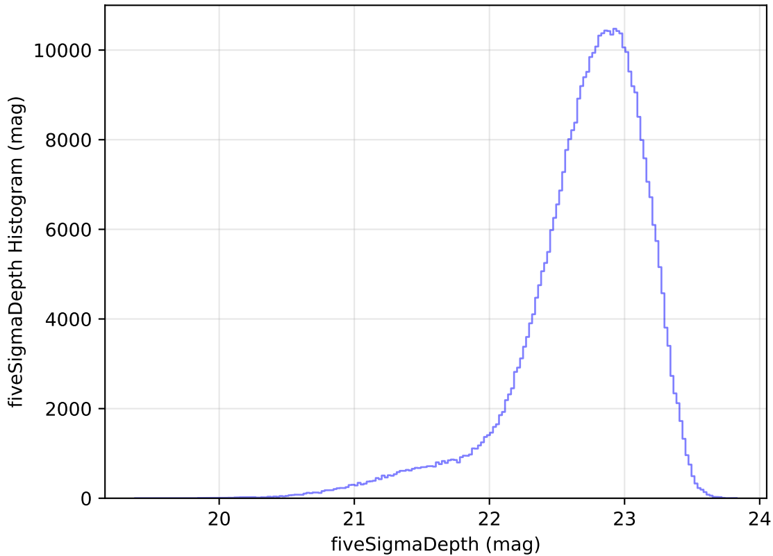
baseline_v3.2_10yrs z: fiveSigmaDepth Histogram
