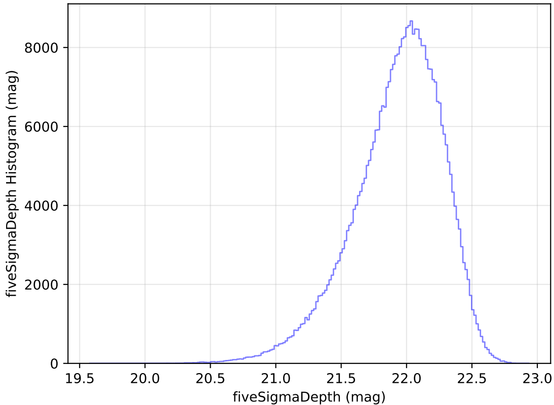
baseline_v3.2_10yrs y: fiveSigmaDepth Histogram
