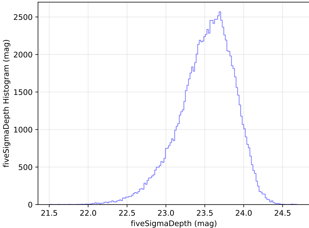
baseline_v3.2_10yrs u: fiveSigmaDepth Histogram
