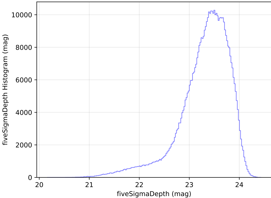
baseline_v3.2_10yrs i: fiveSigmaDepth Histogram
