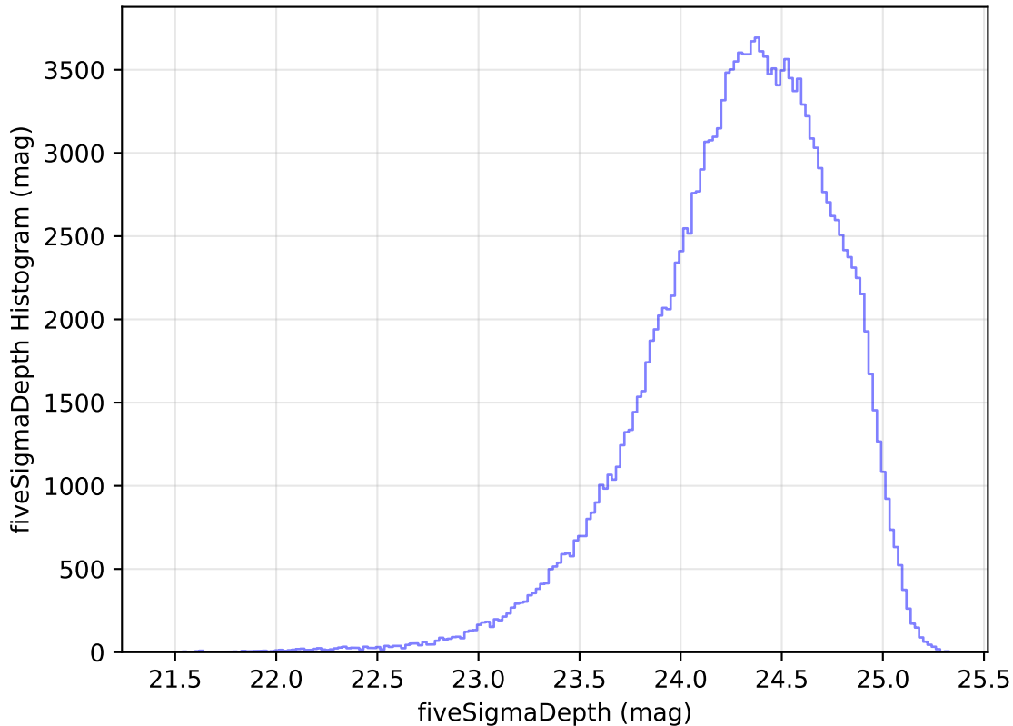
baseline_v3.2_10yrs g: fiveSigmaDepth Histogram
