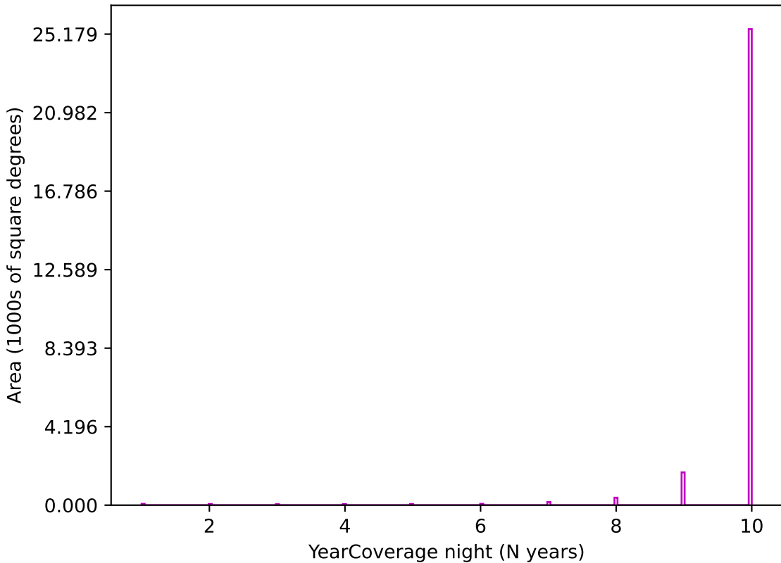
baseline_v3.2_10yrs z band: YearCoverage night
