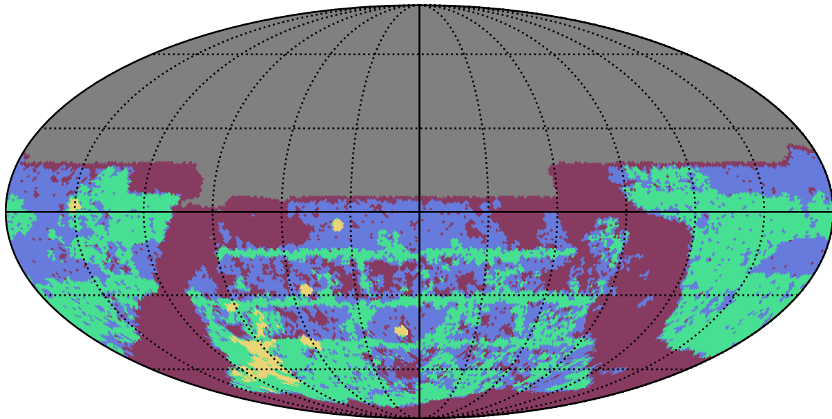
baseline_v3.2_10yrs u band: YearCoverage night
