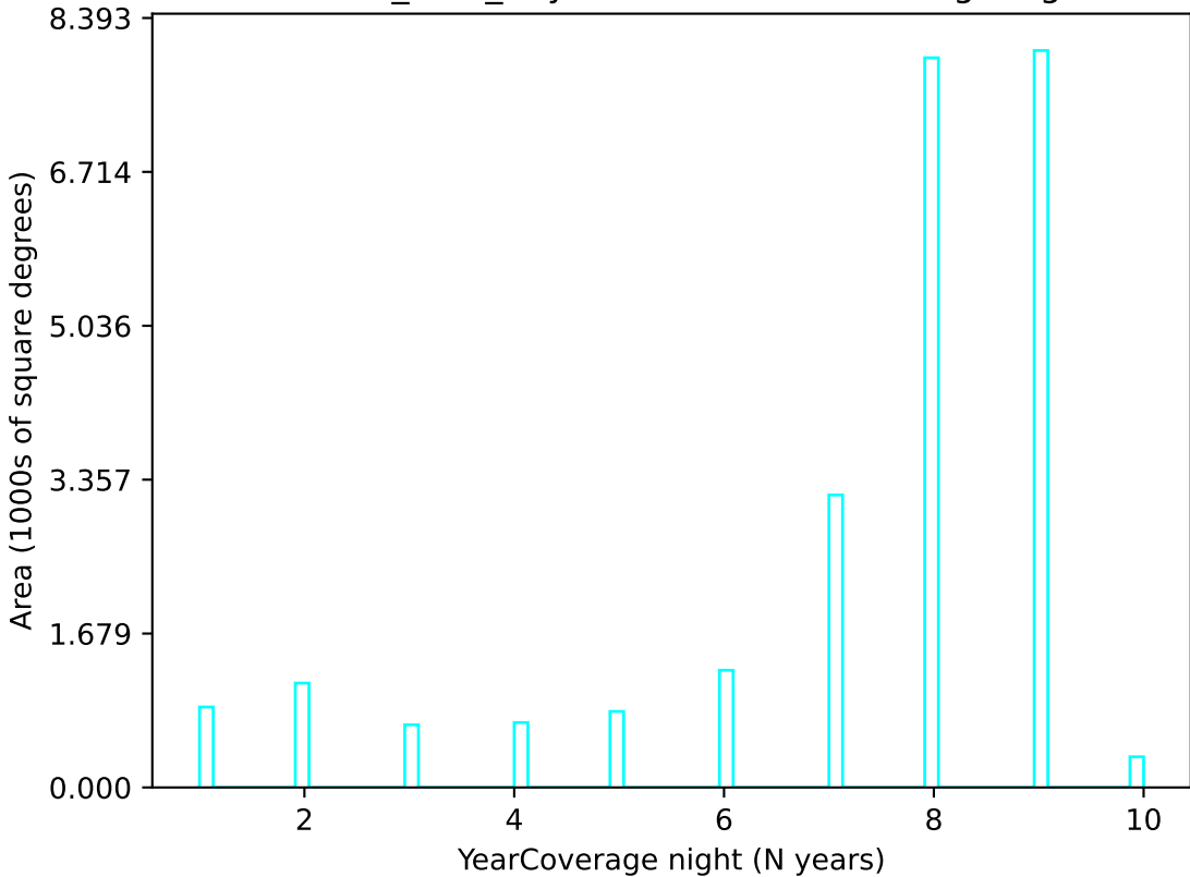
baseline_v3.2_10yrs u band: YearCoverage night
