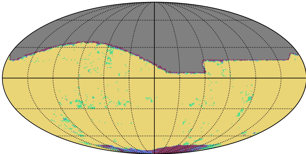
baseline_v3.2_10yrs r band: YearCoverage night
