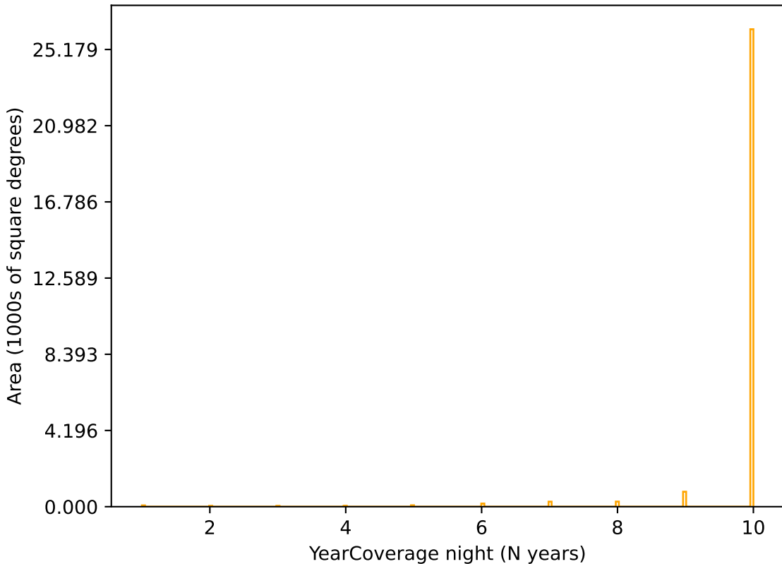
baseline_v3.2_10yrs r band: YearCoverage night
