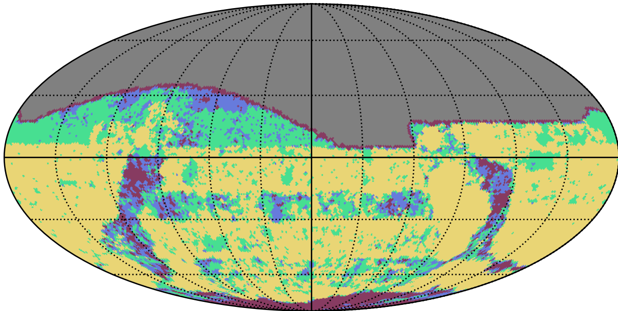
baseline_v3.2_10yrs g band: YearCoverage night
