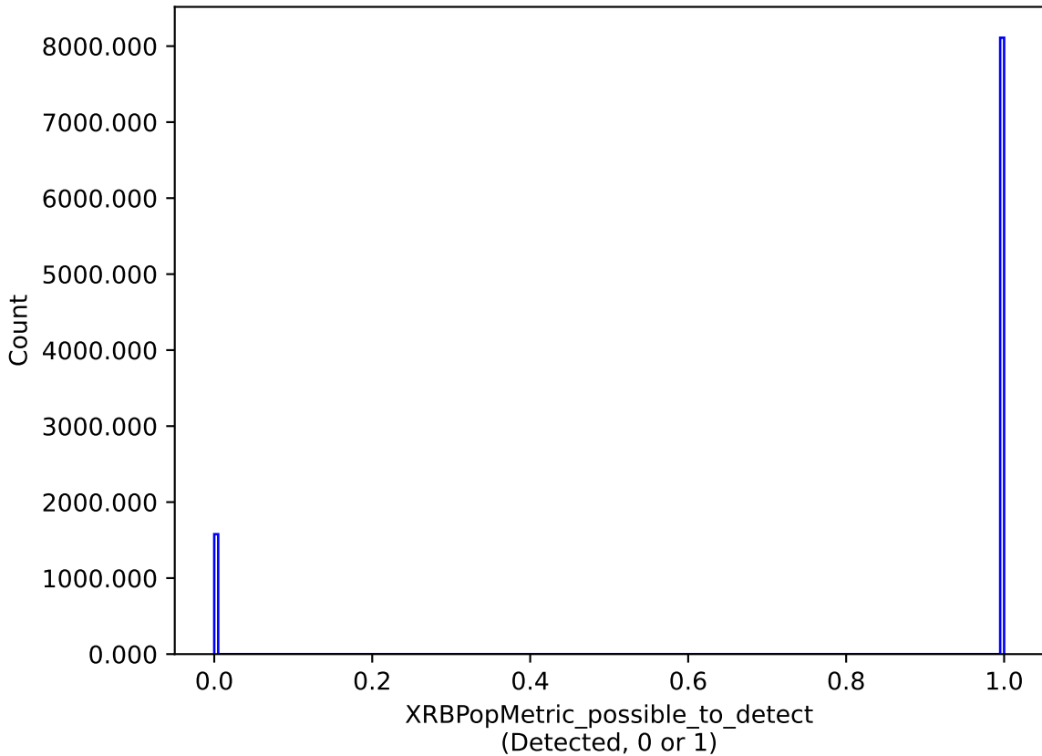
baseline_v3.2_10yrs : XRBPoMetric_possible_to_detect
