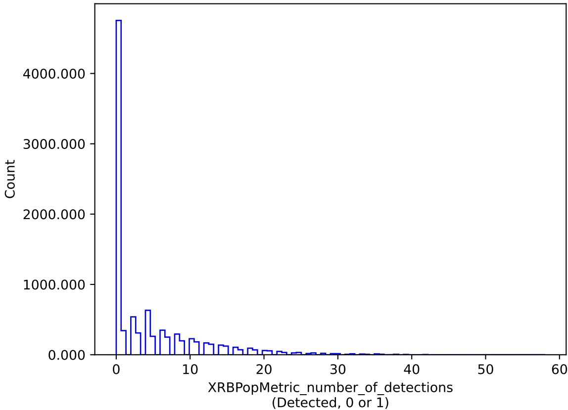
baseline_v3.2_10yrs : XRBPoMetric_number_of_detections
