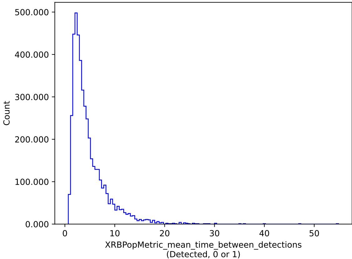
baseline_v3.2_10yrs : XRBPoMetric_mean_time_between_detections
