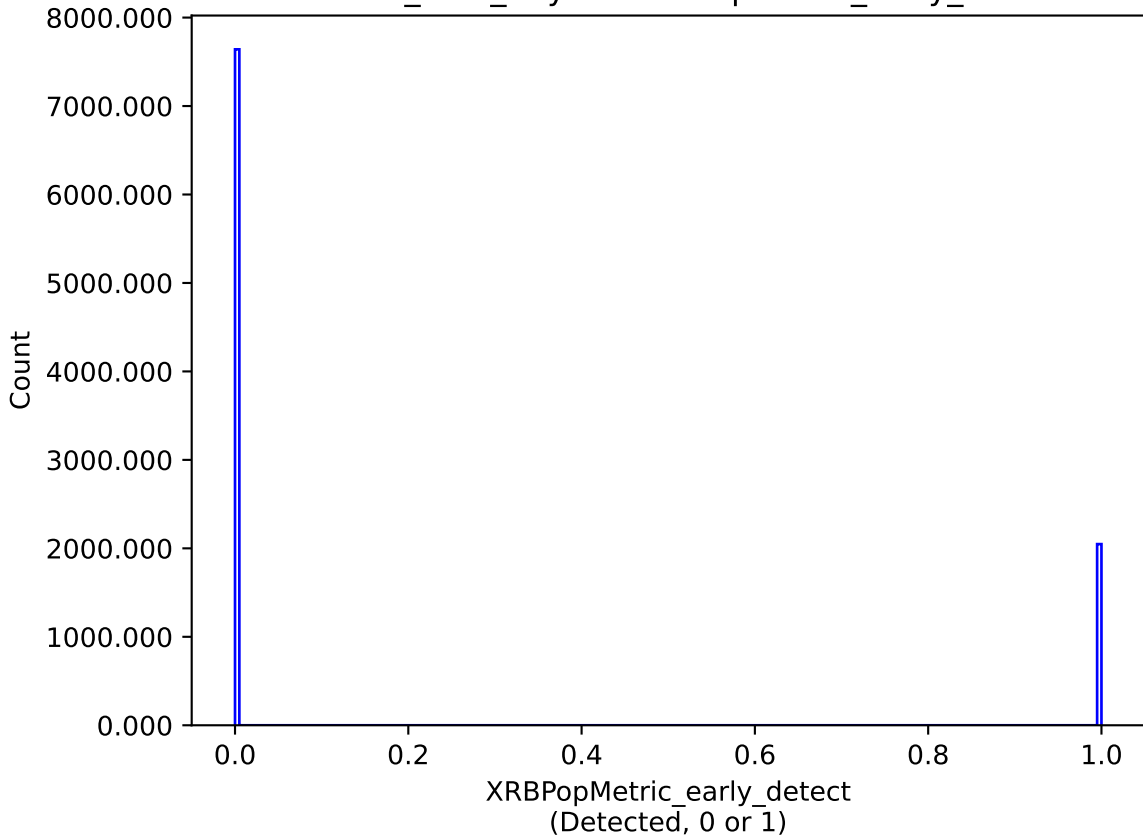
baseline_v3.2_10yrs : XRBPoMetric_early_detect
