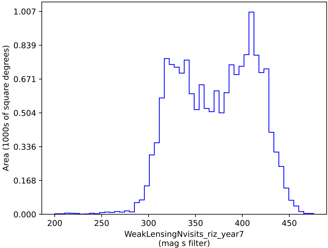
baseline_v3.2_10yrs gri band non-DD: WeakLensingNvisits_riz_year7
