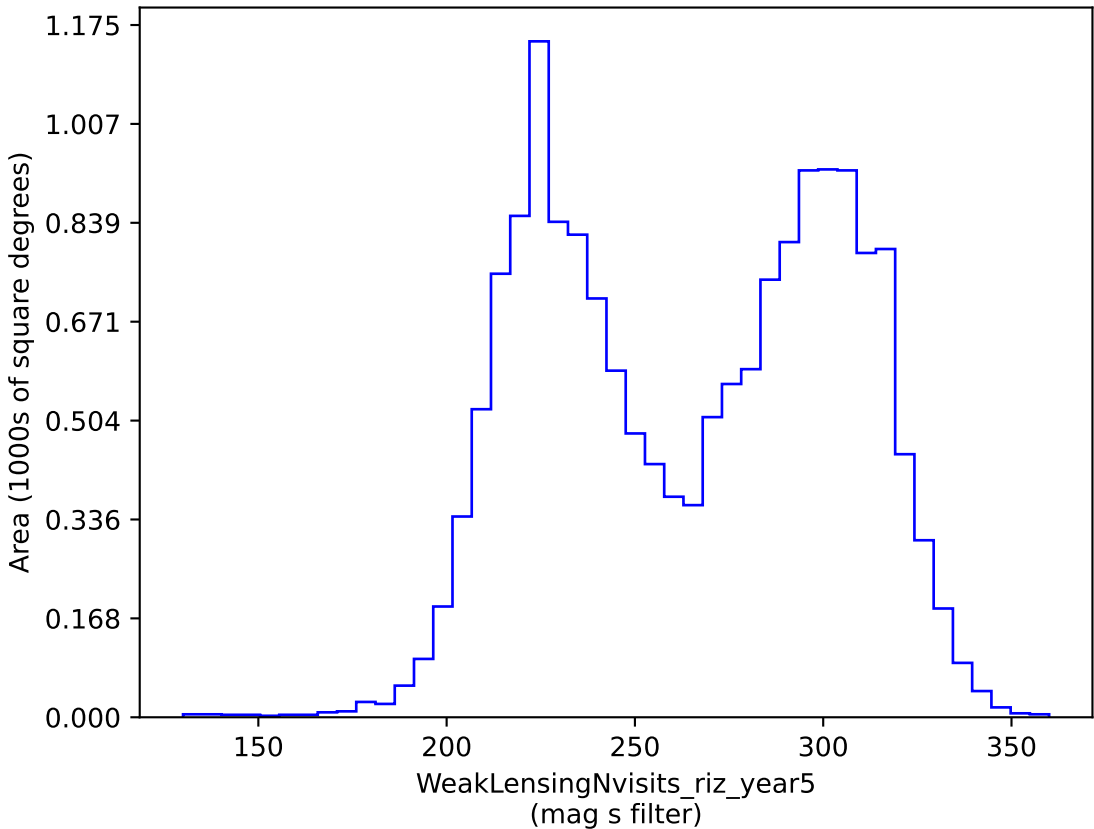
baseline_v3.2_10yrs gri band non-DD: WeakLensingNvisits_riz_year5
