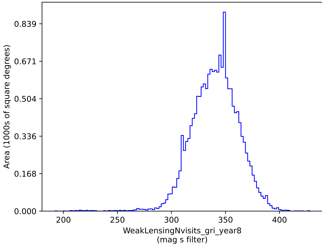
baseline_v3.2_10yrs gri band non-DD: WeakLensingNvisits_gri_year8
