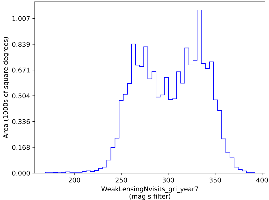
baseline_v3.2_10yrs gri band non-DD: WeakLensingNvisits_gri_year7
